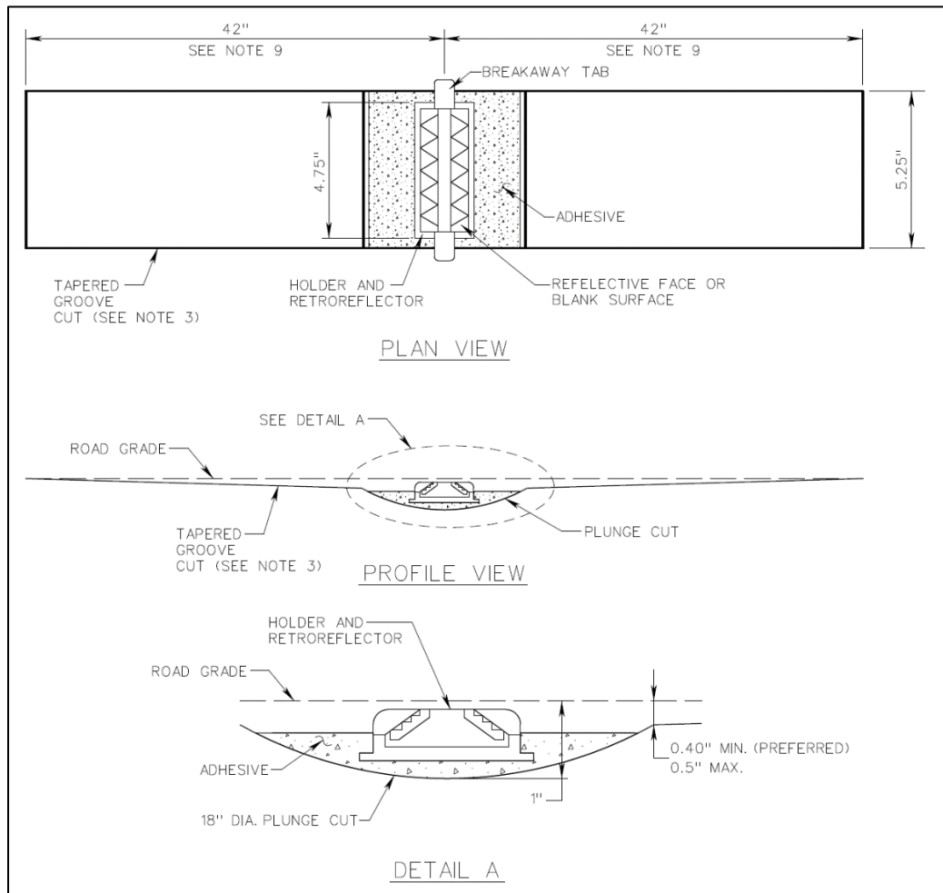
Figure 1: Installation of Inlaid Pavement Marker
